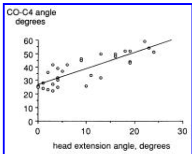
Figure 5. Comparison of the head extension angle with the angle between the occiput and C4 (C0-C4 angle). The C0-C4 angle is the angle measured between the C0 and C4 reference lines on the radiograph. Data are included for arytenoid exposure and best view for both the Macintosh and Bullard laryngoscopes. Head extension angle correlated significantly with C0-C4 angle ( r^2 0.7). Regression line: head extension angle 27 + 1.19 \times \text{C0-C4 angle} . Head extension angle also was correlated with the angles at C0-C1 and C1-C2 (data not shown).
